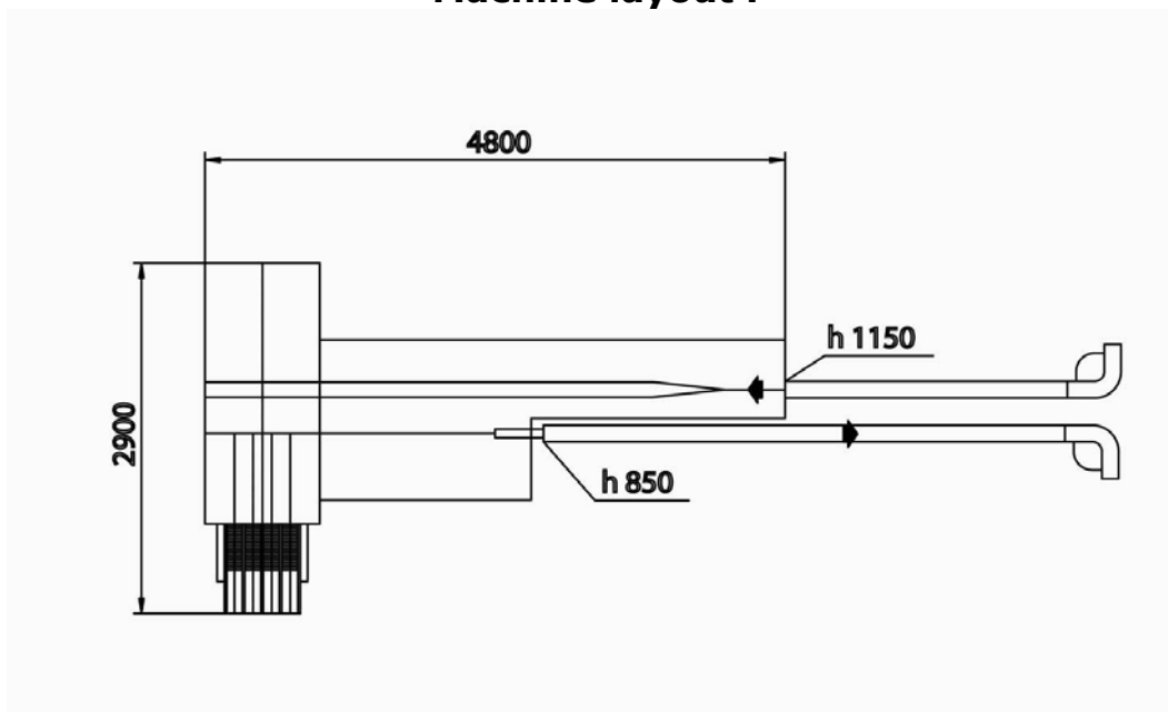
Machine layout .
